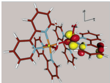
Figure 1. Metal-dominated broken symmetry MO ( \alpha -spin) that promotes antiferromagnetic coupling. Isosurface drawn at 0.05 au.
